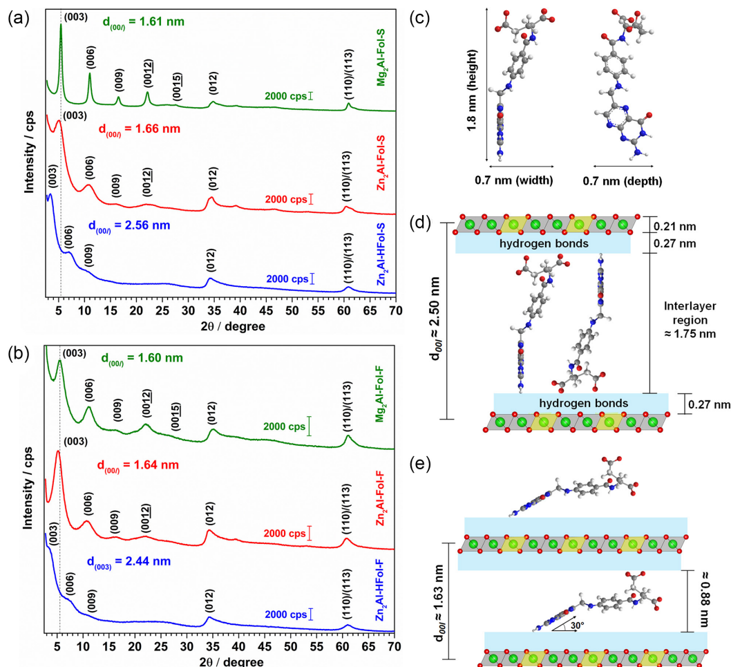
Figure 2. XRD patterns of powdered samples obtained by slow coprecipitation (a) and fast coprecipitation (b); folate dimensions estimated by Chem3D Pro software 28 (c); arrangement proposed for HFOl^{2-} intercalated into Zn_2Al-HFOl-S and Zn_2Al-HFOl-F samples (d); arrangement proposed for Fol^{3-} intercalated into Mg_2Al-Fol-S , Mg_2Al-Fol-F , Zn_2Al-Fol-S and Zn_2Al-Fol-F samples (e). The arrangement of folate anions was proposed, considering the arrangement of molecules in the crystal structure of dihydrate FA resolved by Kaduk et al. 29
